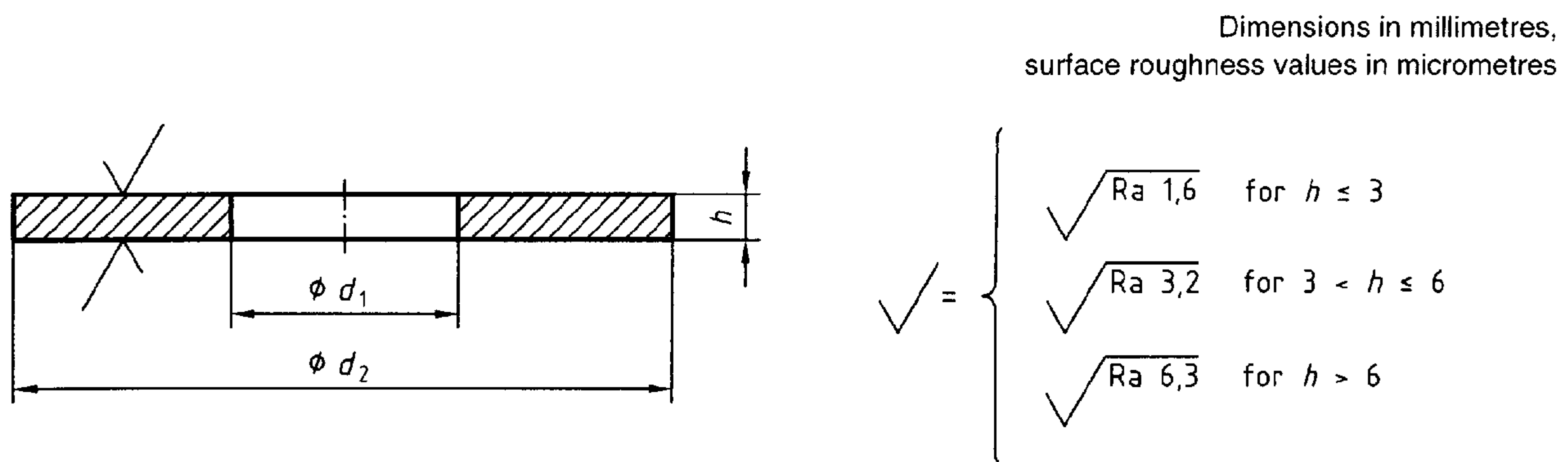
Figure 1 — Dimensions
